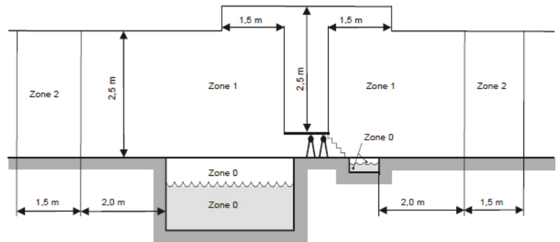
>> Swimming pool zones as specified in the International safety standard IEC 60364-7-702
