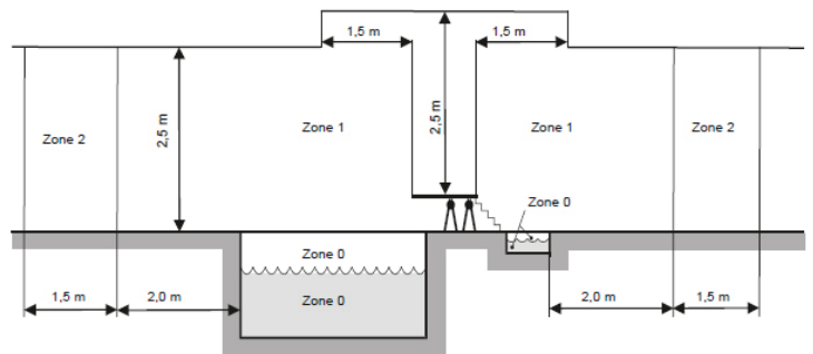
>> Swimming pool zones as specified in International standard IEC 60364-7-702
